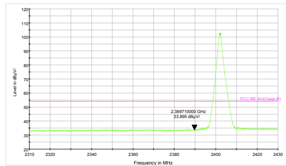
DH5-Channel 0: Average
