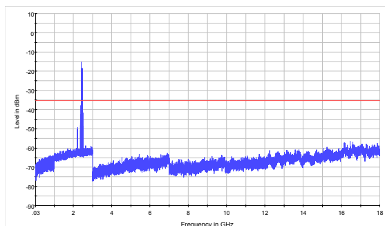
GFSK-CH3930MHz to 18GHz
