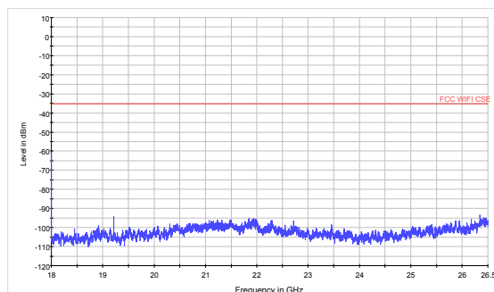
GFSK -CH39 18GHz to 26.5GHz
