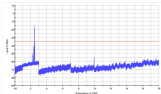
EDR-CH030MHz to 18GHz
