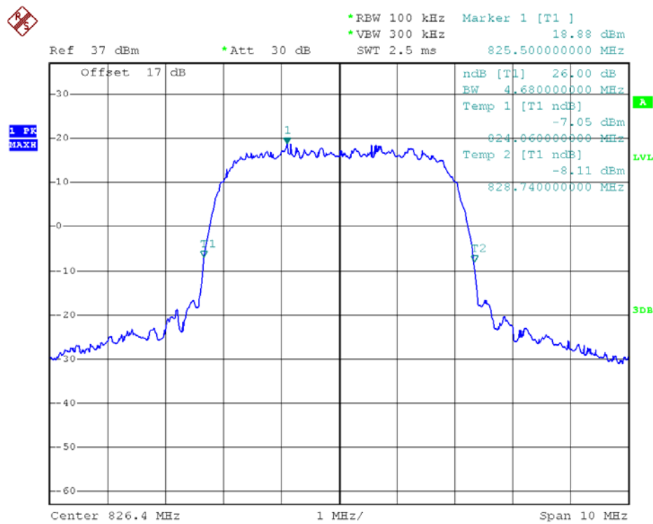
(Plot E1: WCDMA 850MHz Channel = 4132 26dB bandwidth)
