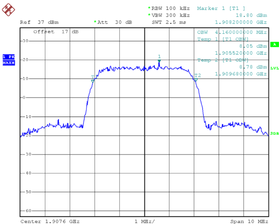
(Plot F6: WCDMA 1900MHz Channel = 9538 99% Occupied Bandwidth)
