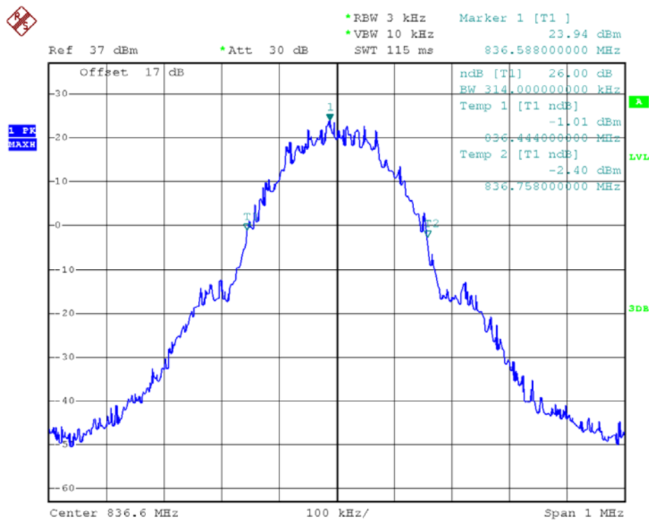
(Plot A3: GSM 850MHz Channel = 190 26dB bandwidth)
