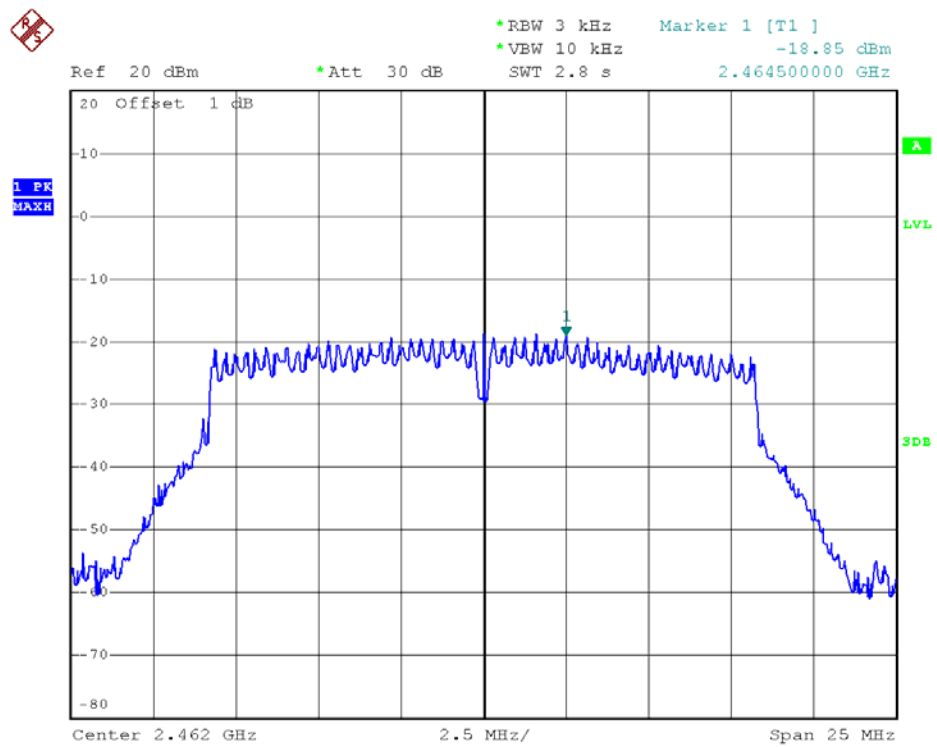
802.11g - Channel 11
