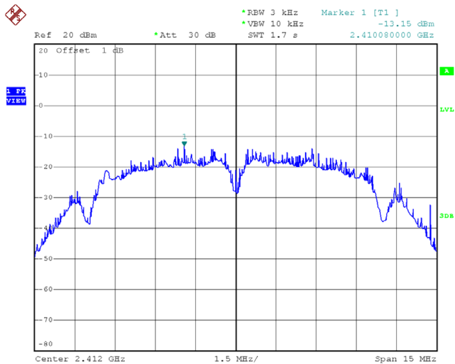
802.11b - Channel 1
