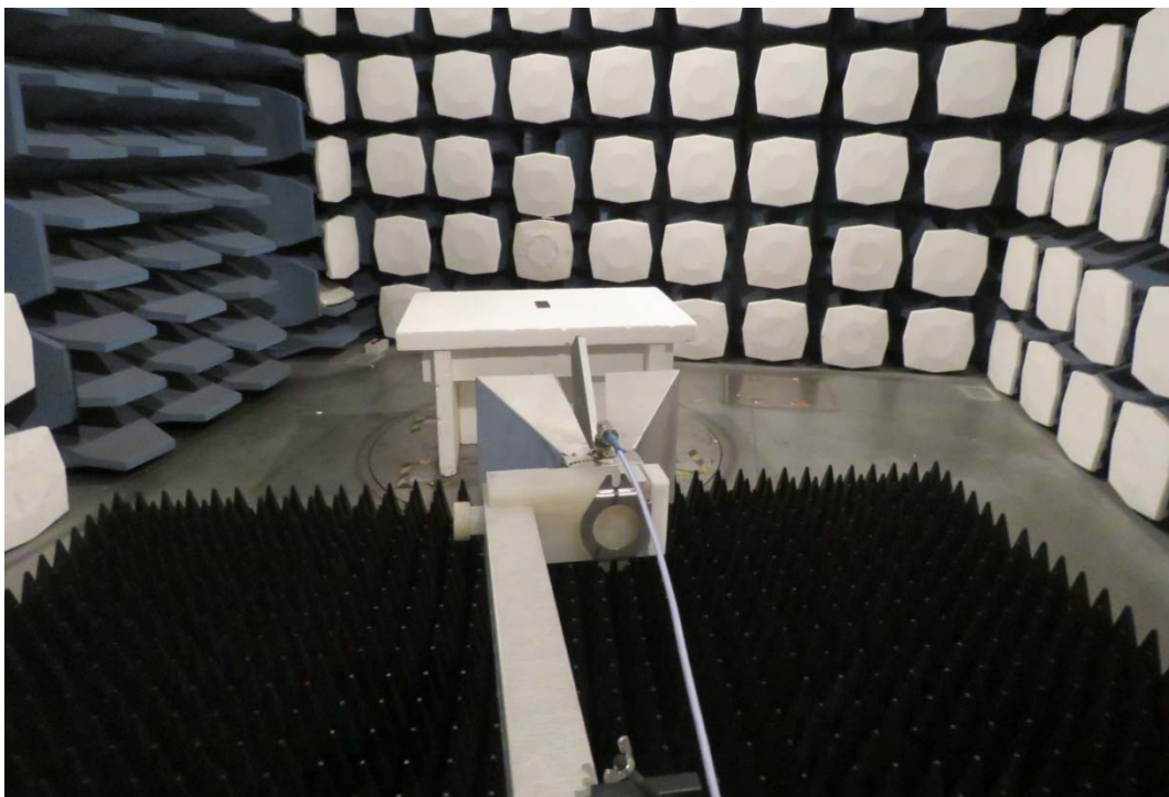
Picture 1: Radiated Spurious Emissions Test setup
