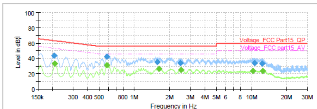
BT_L_0.15-30Mhz
