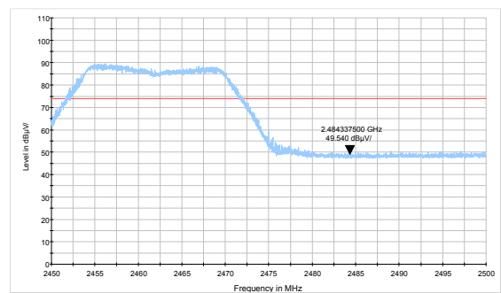
802.11g-Channel 11: Peak
