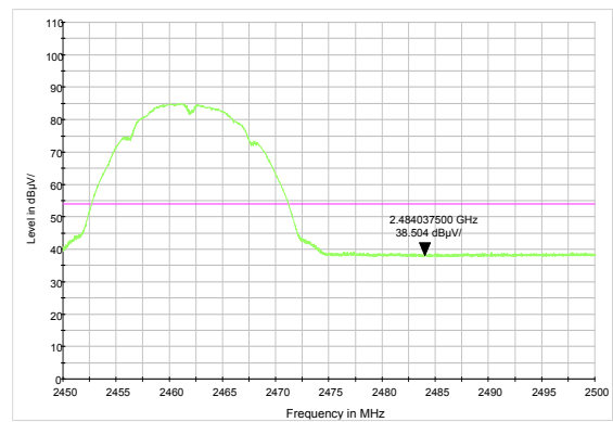
802.11g-Channel 11: Peak
