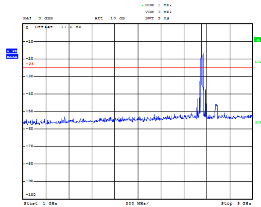
LTE Band 7 20MHz CH-High 1GHz~3GHz
