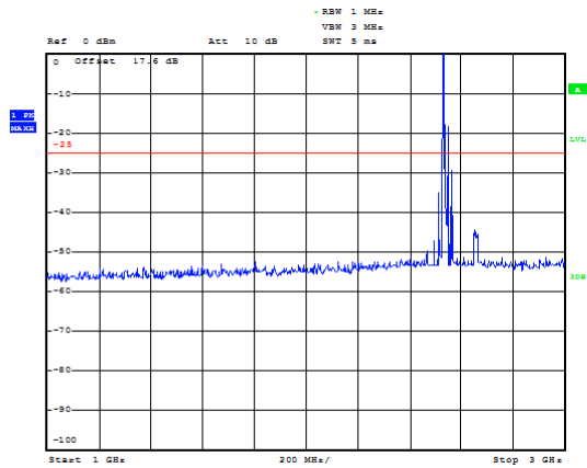
LTE Band 7 20MHz CH-Middle 1GHz~3GHz
