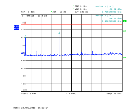
GSM 1900 CH-Middle 3GHz~20GHz
