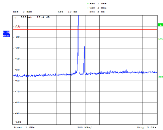
LTE Band 2 5MHz CH-High 1GHz~3GHz
