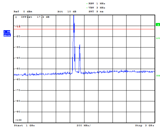
LTE Band 2 10MHz CH-Low 1GHz~3GHz
