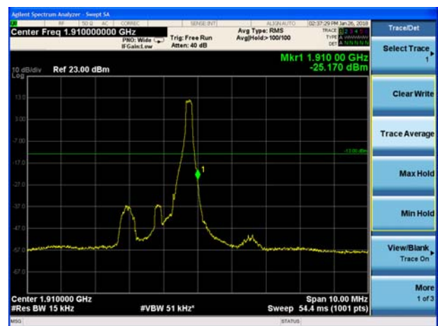
LTE Band 2 1.4MHz 16QAM 100%RB CH-High
