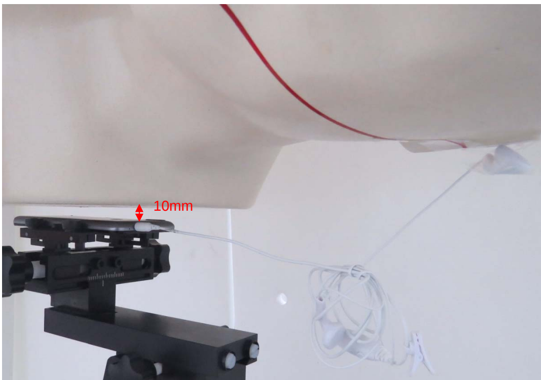
Picture 12: Back Side with Earphone 1, the distance from handset to the bottom of the Phantom is 10mm
