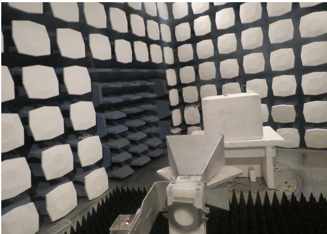
Picture 1 Radiated Emission Test Setup
