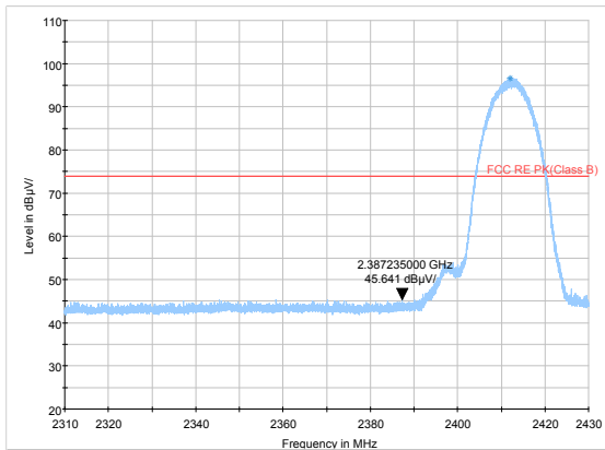
802.11b-Channel 1: Peak
