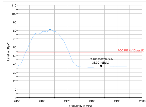
802.11b-Channel 11: Average
