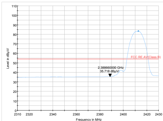
802.11b-Channel 1: Average
