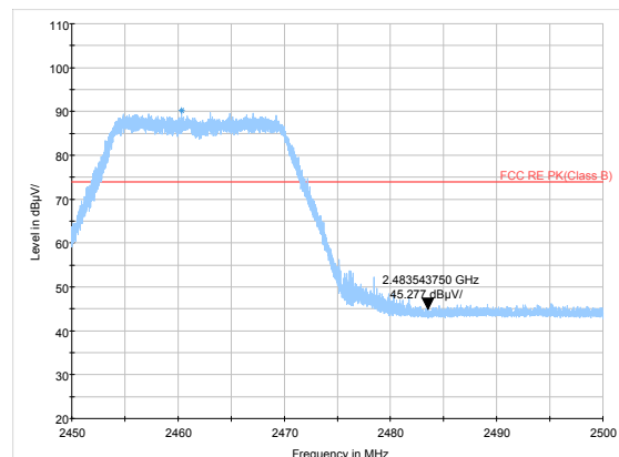
802.11g-Channel 11: Peak
