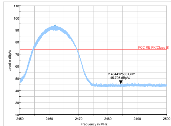
802.11b-Channel 11: Peak
