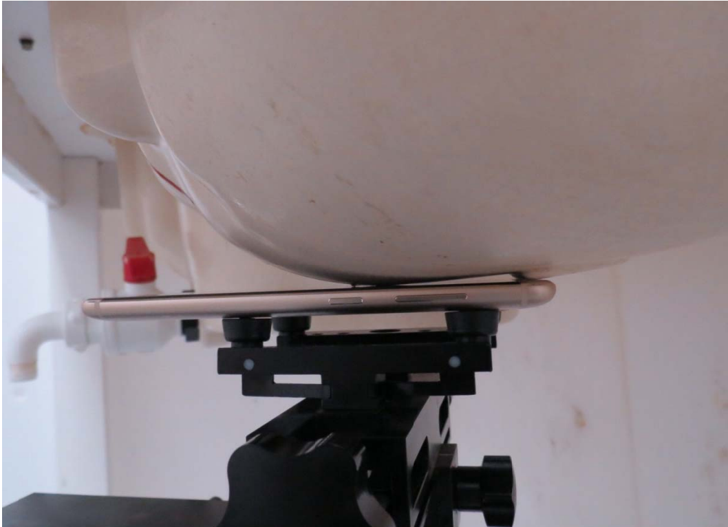
Picture 16: Left Hand Touch Cheek Position
