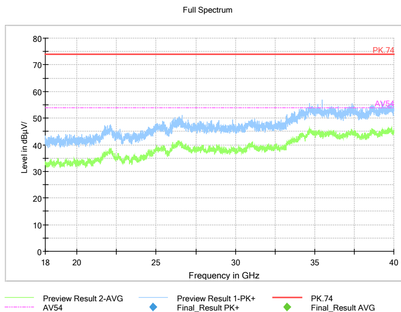
Pic8. Radiated emission (18GHz –40GHz)
