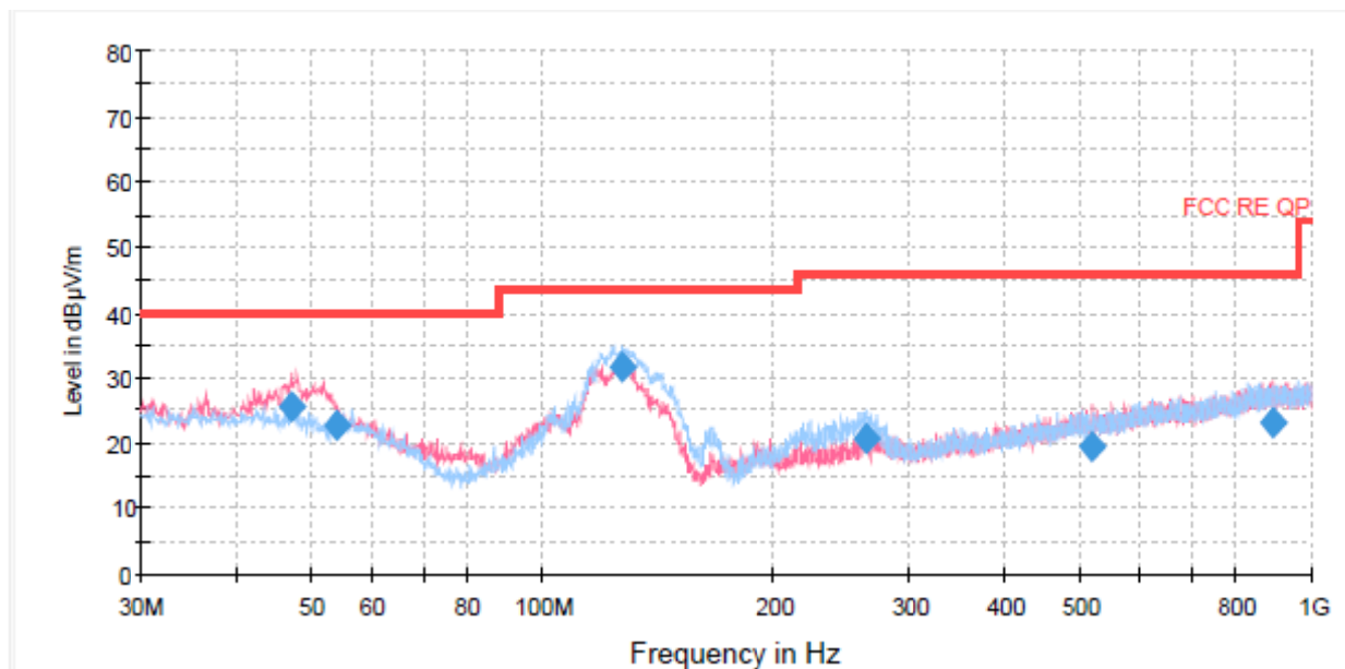
Radiates Emission from 30MHz to 1GHz
