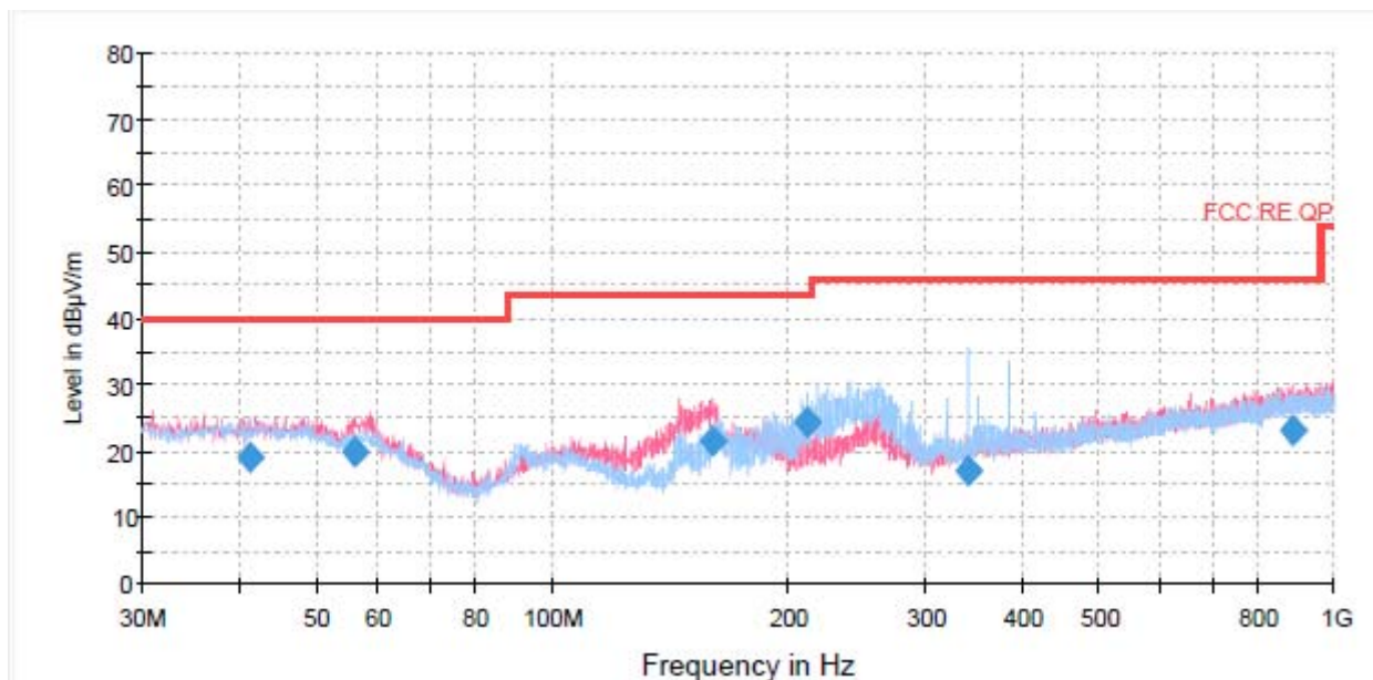
Radiated Emission from 30MHz to 1GHz
