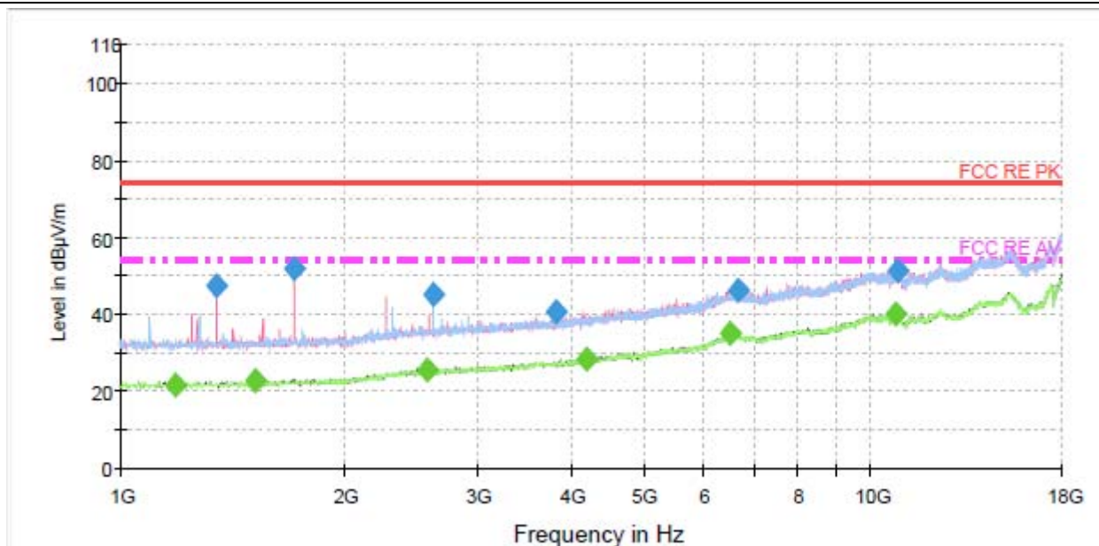
Radiated Emission from 1GHz to 18GHz
