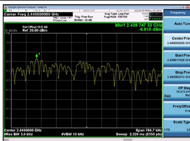
Power spectral density: 2440MHz
