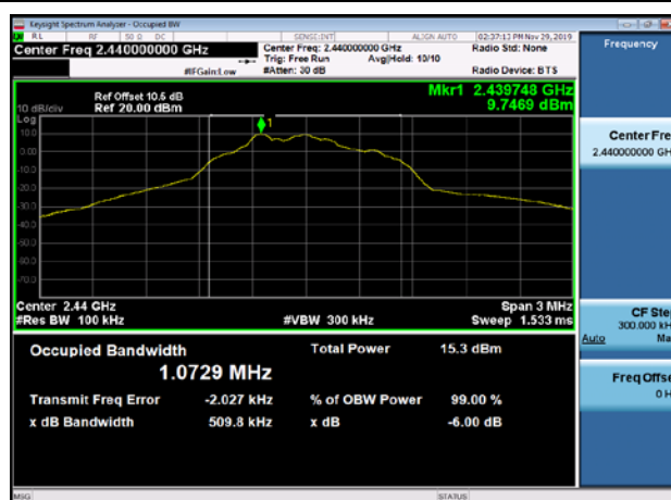
6dB Bandwidth: 2440MHz
