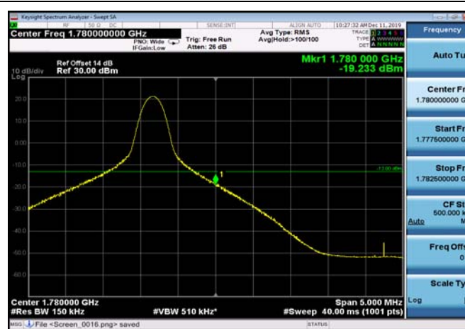
HighRange_FDD66_15MHz_1772.5_OneRB _high_QPSK
