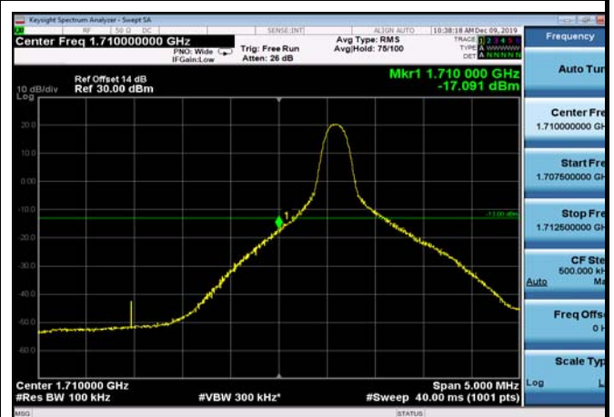
LowRange_FDD66_10MHz_1715_fullRB _Low_Q16
