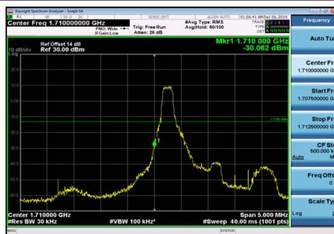
LowRange_FDD66_1.4MHz_1710.7_fullRB _Low_QPSK
