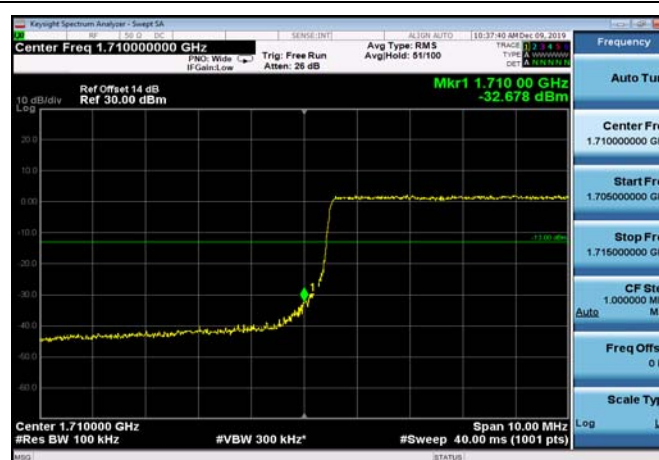
LowRange_FDD66_15MHz_1717.5_OneRB
