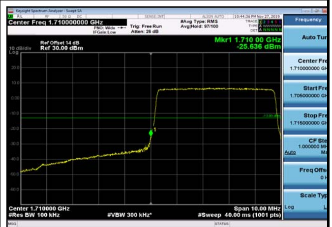
LowRange_FDD66_10MHz_1715_OneRB _low_Q16
