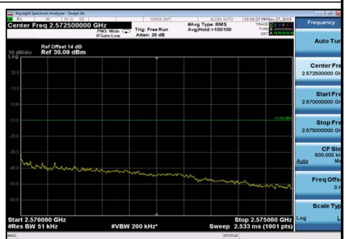
FDD07_5MHz_2567.5_QPSK_fullRB_ExtraBa nds_Range_2570~2575
