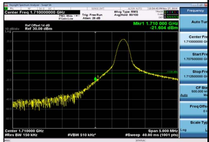
LowRange_FDD66_15MHz_1717.5_fullRB _Low_Q16
