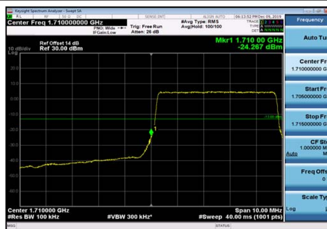
LowRange_FDD66_10MHz_1715_OneRB _low_QPSK
