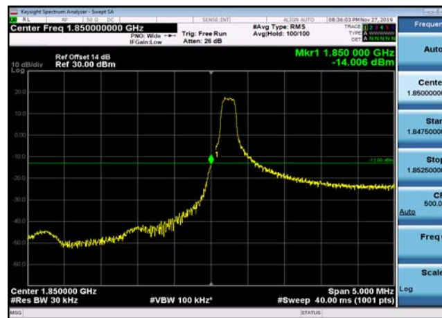
LowRange_FDD02_3MHz_1851.5_fullRB _Low_QPSK
