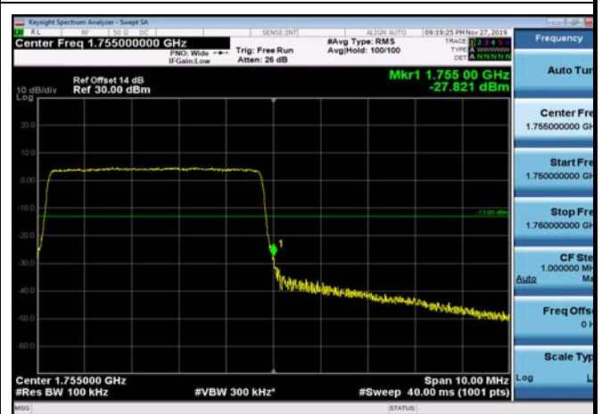
HighRange_FDD04_10MHz_1750_OneRB _high_Q16
