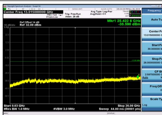
FDD66_LowRange_20MHz_30MHz~26GHz
