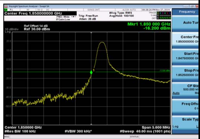
LowRange_FDD02_5MHz_1852.5_OneRB _low_Q16
