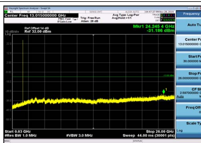
FDD66_HighRange_15MHz_30MHz~26GHz
