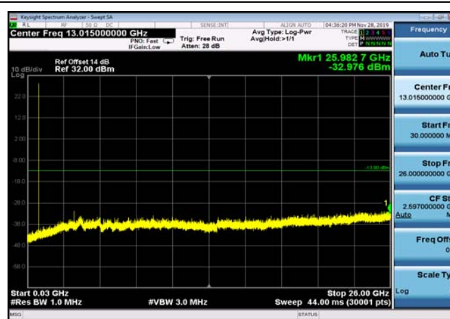
FDD05_HighRange_3MHz_30MHz~26GHz
