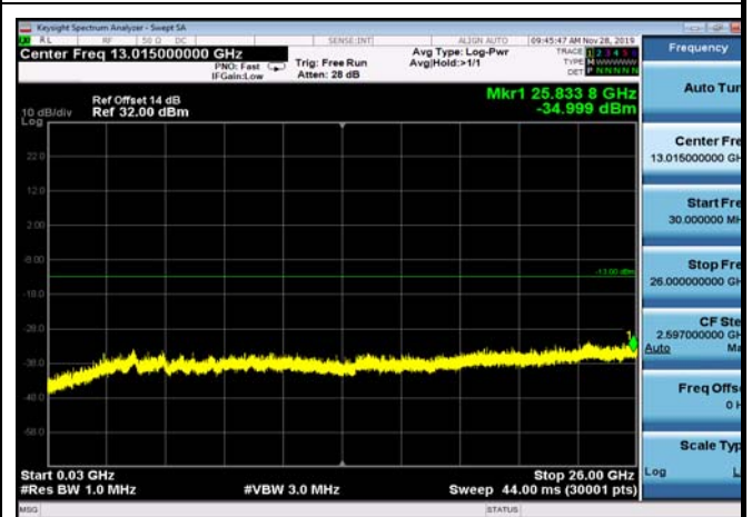
FDD66_LowRange_30MHz_30MHz~26GHz
