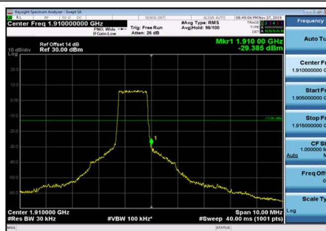
HighRange_FDD02_1.4MHz_1909.3 _fullRB_High_QPSK
