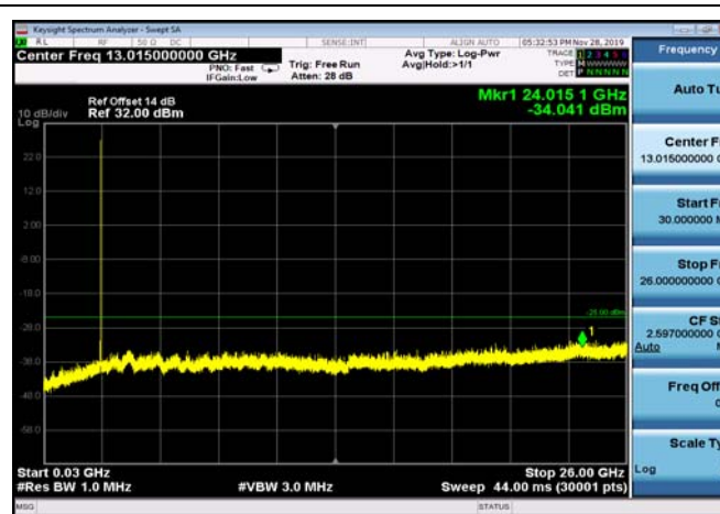
FDD07_HighRange_20MHz_30MHz~26GHz
