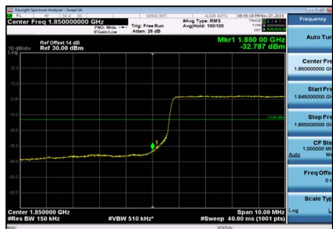
LowRange_FDD02_20MHz_1860_OneRB _low_Q16
