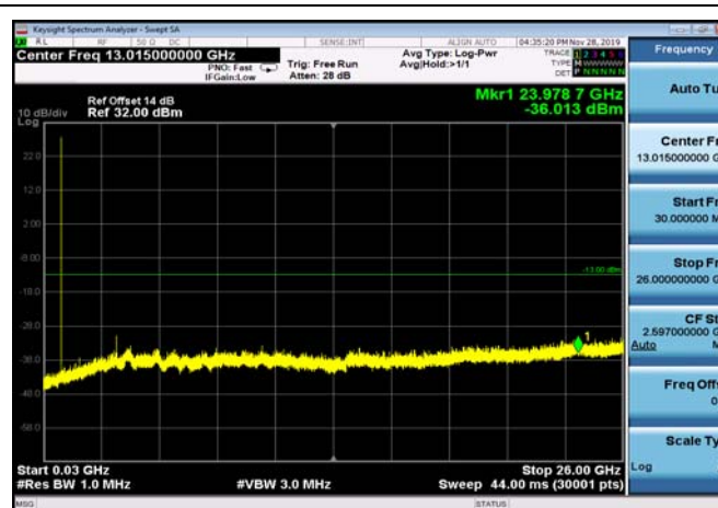
FDD05_LowRange_1.4MHz_30MHz~26GHz
