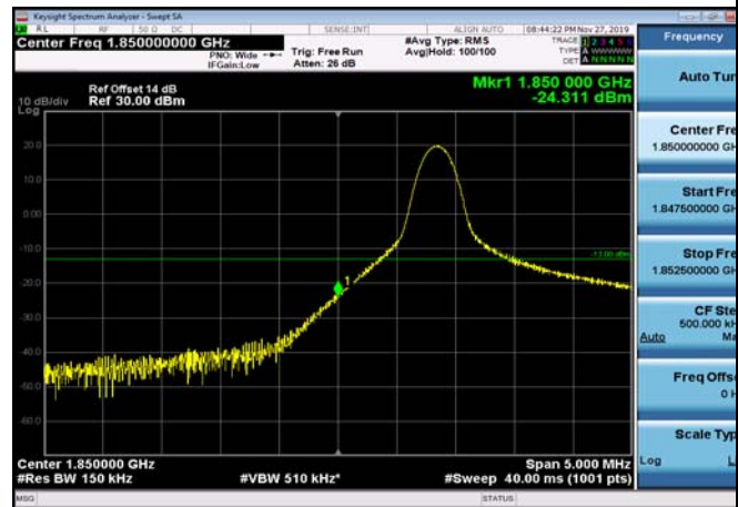
LowRange_FDD02_15MHz_1857.5_fullRB _Low_Q16
