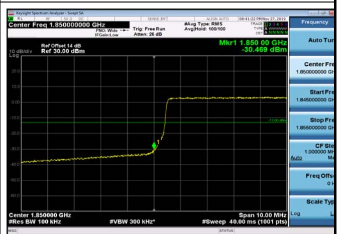
LowRange_FDD02_10MHz_1855_fullRB _Low_Q16
