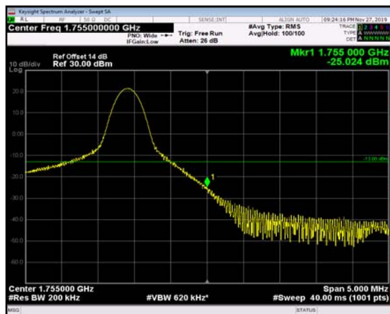
HighRange_FDD04_20MHz_1745_OneRB _high_QPSK
