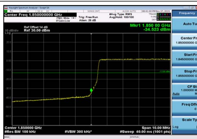
LowRange_FDD02_10MHz_1855_fullRB _Low_QPSK
