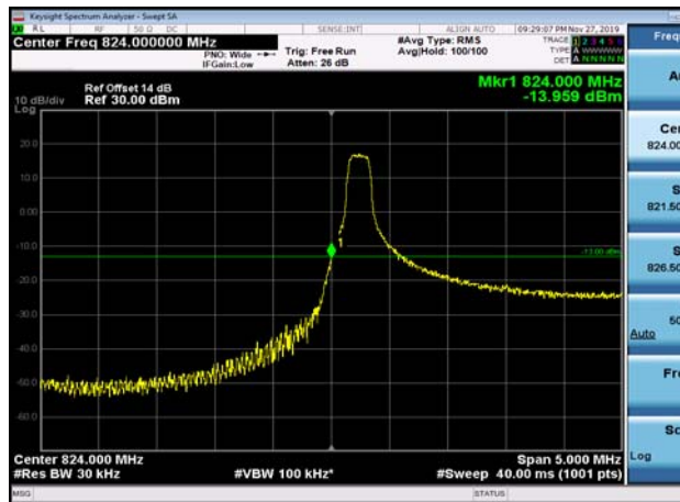
LowRange_FDD05_3MHz_825.5_fullRB _Low_QPSK
