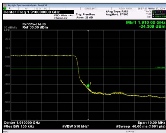
HighRange_FDD02_20MHz_1900_OneRB _high_QPSK
