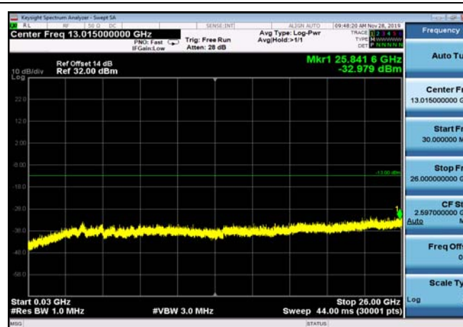
FDD66_HighRange_3MHz_30MHz~26GHz
