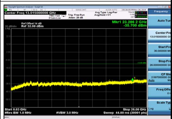
FDD66_HighRange_20MHz_30MHz~26GHz
