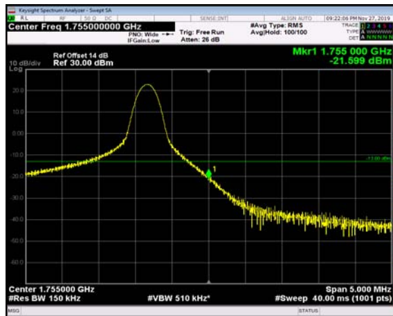
HighRange_FDD04_15MHz_1747.5_fullRB _High_QPSK
