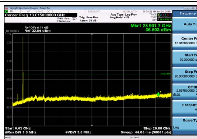
FDD66_MidRange_20MHz_30MHz~26GHz
