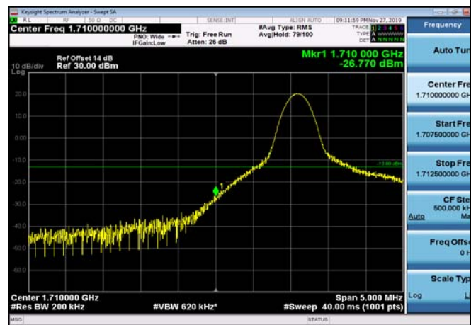
LowRange_FDD04_20MHz_1720_OneRB _low_Q16
