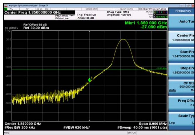
LowRange_FDD02_20MHz_1860_OneRB _low_Q16
