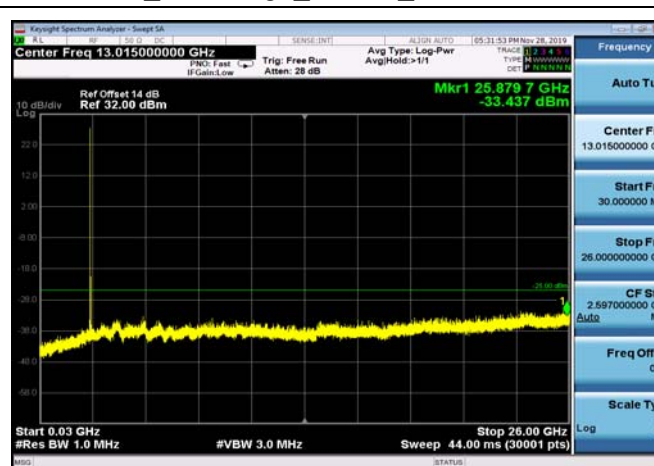
FDD07_LowRange_10MHz_30MHz~26GHz
