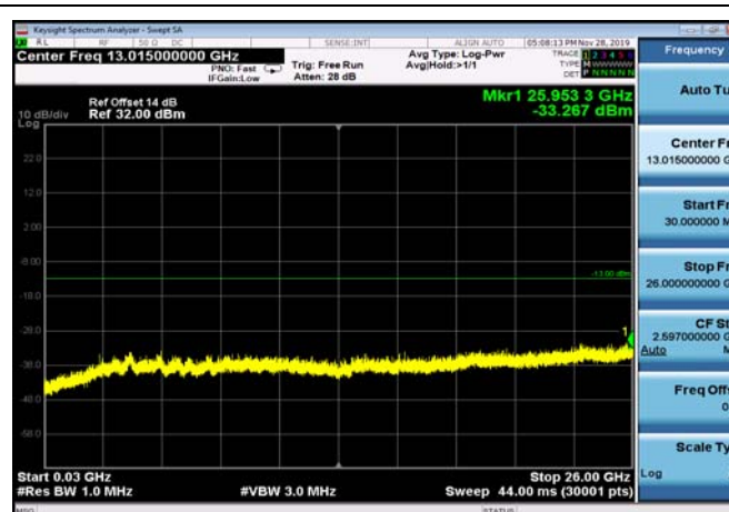
FDD66_LowRange_5MHz_30MHz~26GHz
