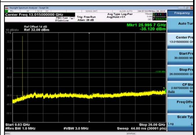
FDD66_MidRange_3MHz_30MHz~26GHz
