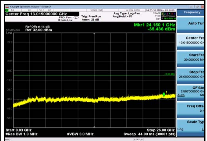
FDD66_MidRange_1.4MHz_30MHz~26GHz
