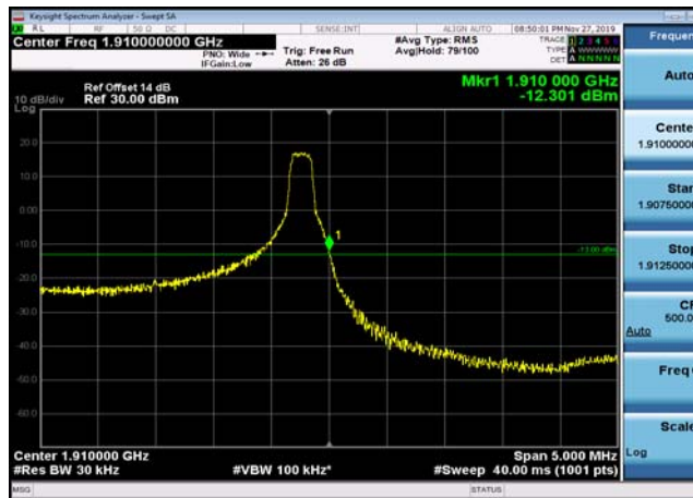
HighRange_FDD02_3MHz_1908.5_fullRB _High_QPSK
