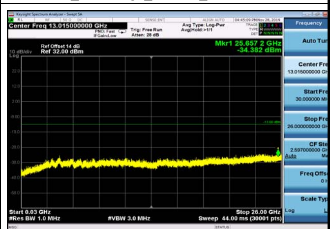
FDD66_LowRange_1.4MHz_30MHz~26GHz
