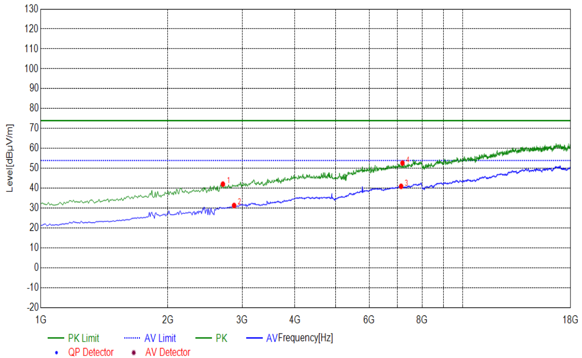
(Plot M: Test Antenna Horizontal 1G – 18G)
