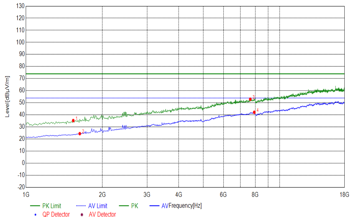
(Plot N: Test Antenna Vertical 1G – 18G)
