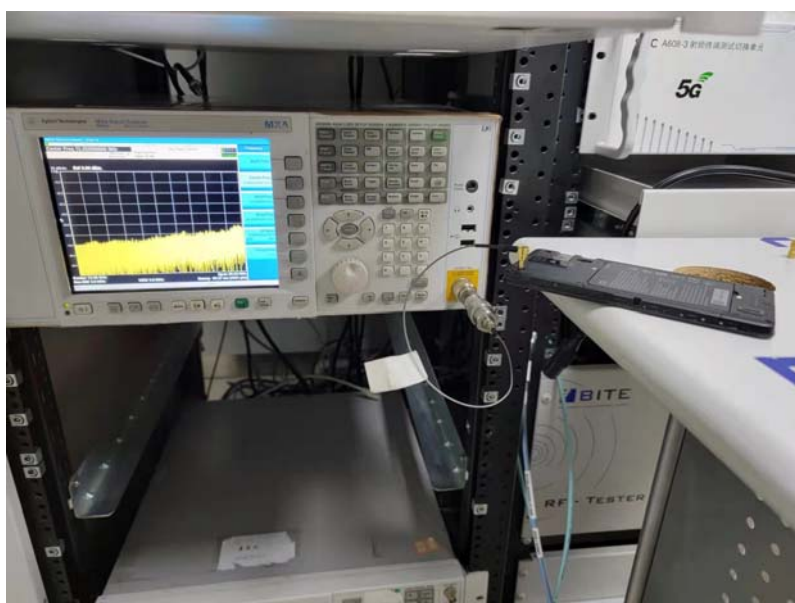
RF Conducted Test setup (BT/WIFI)
