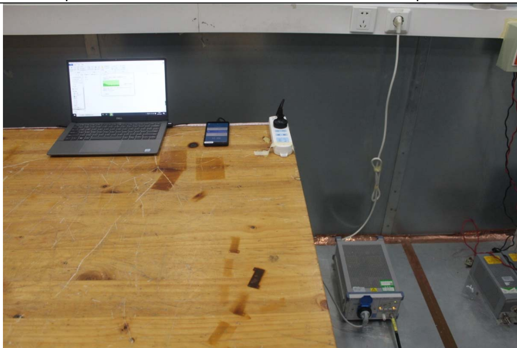
Picture 1: Conducted Emissions Test Setup
