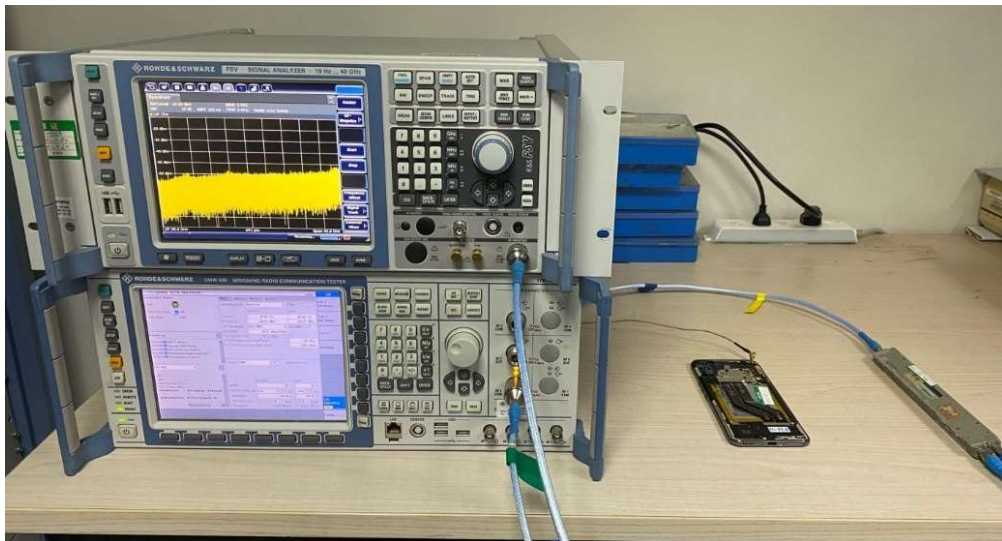
RF Conducted Test
