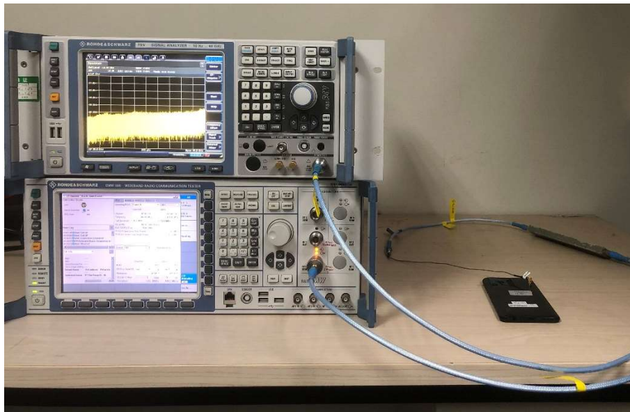
RF Conducted Test
