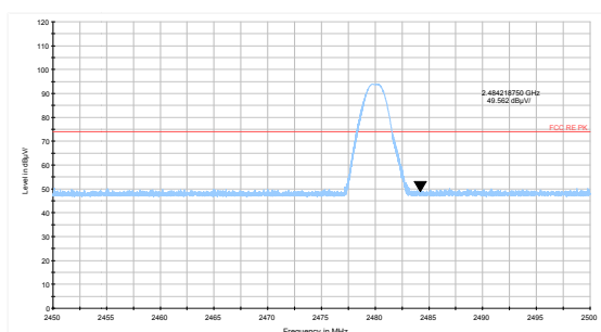
DH5-Channel 78: Peak
