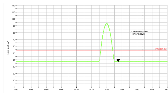
DH5-Channel 78: Average
