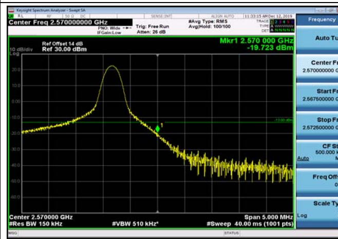
HighRange_FDD07_15MHz_2562.5_OneRB _high_QPSK
