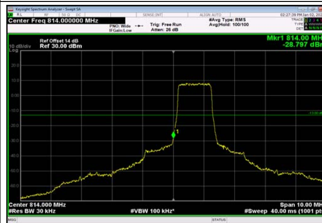
LowRange_FDD26_3MHz_815.5_OneRB _low_QPSK
