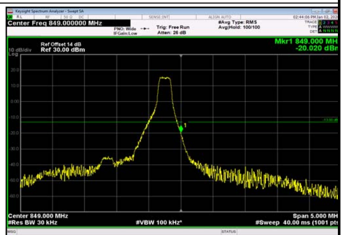
HighRange_FDD26_1.4MHz_848.3_fullRB _High_Q16
