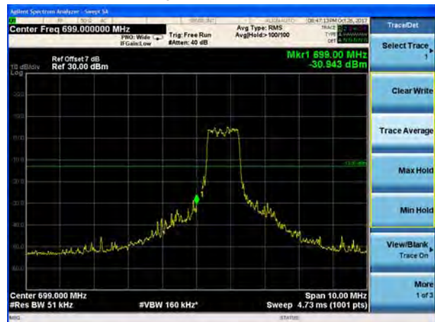
LTE Band 12 16QAM 3MHz CH-Low, 100%RB
