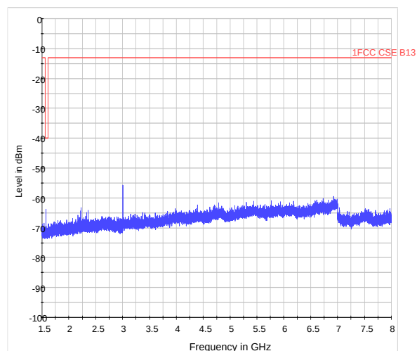
LTE Band 13 10MHz CH- High 1.5GHz~8GHz
