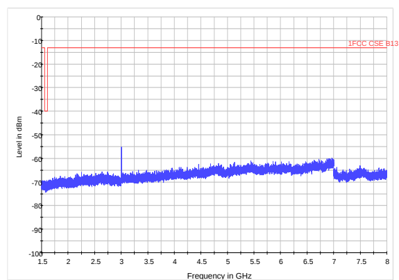
LTE Band 13 10MHz CH- High 1.5GHz~8GHz
