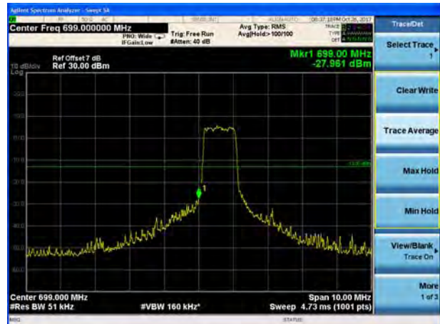
LTE Band 12 16QAM 3MHz CH-Low, 1 RB
