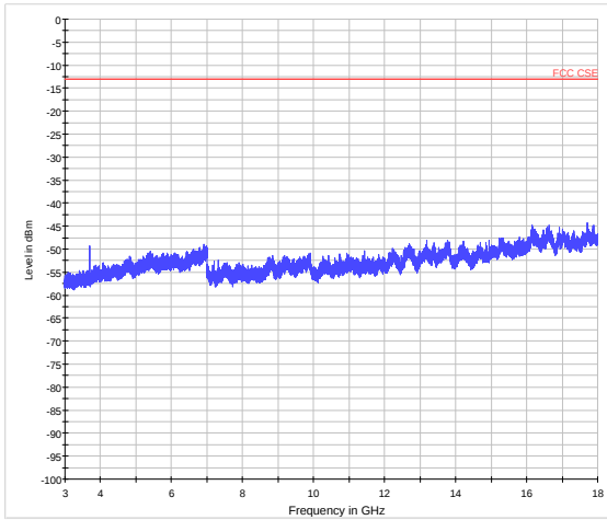
NB-IOT Band 2 CH-Low 3GHz~18GHz
