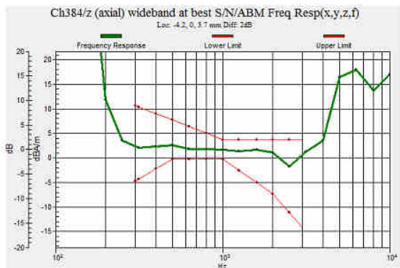
Fig 7.1 CDMA2000 BC0 Ch384
