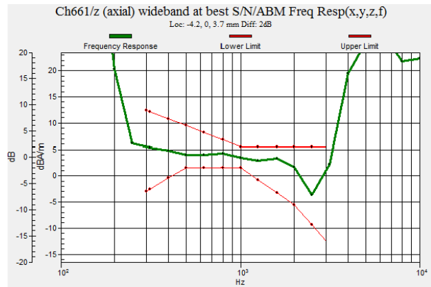
Fig 7.2 GSM1900 Ch661
