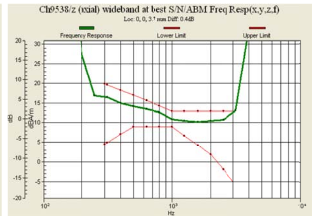
Fig. 8.16 WCDMA Band II Ch9538
