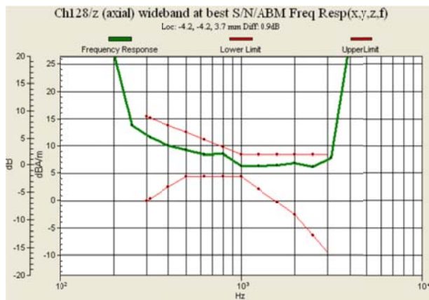
Fig 8.1 GSM850 Ch128
