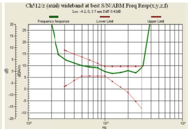
Fig 8.4 GSM1900 Ch512
