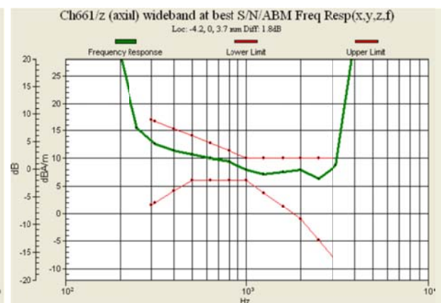
Fig 8.6 GSM1900 Ch661
