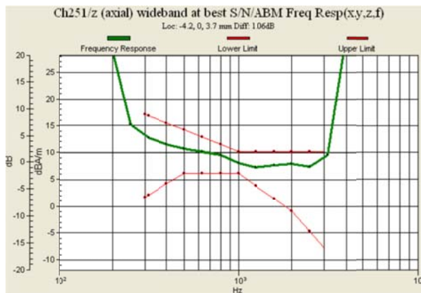
Fig 8.3 GSM850 Ch251
