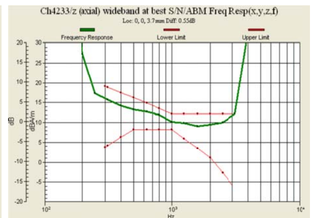
Fig. 8.10 WCDMA Band V Ch4233
