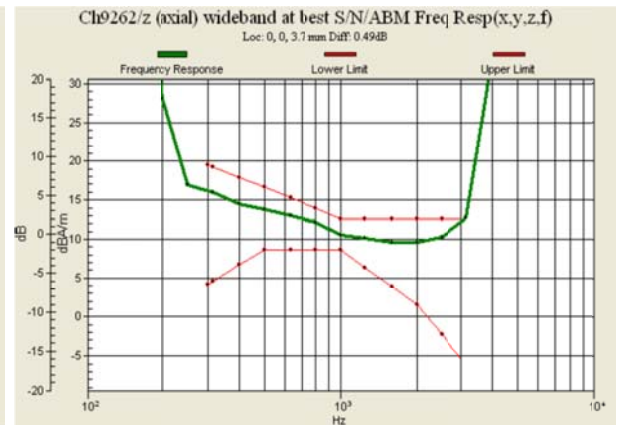
Fig. 8.14 WCDMA Band II Ch9262
