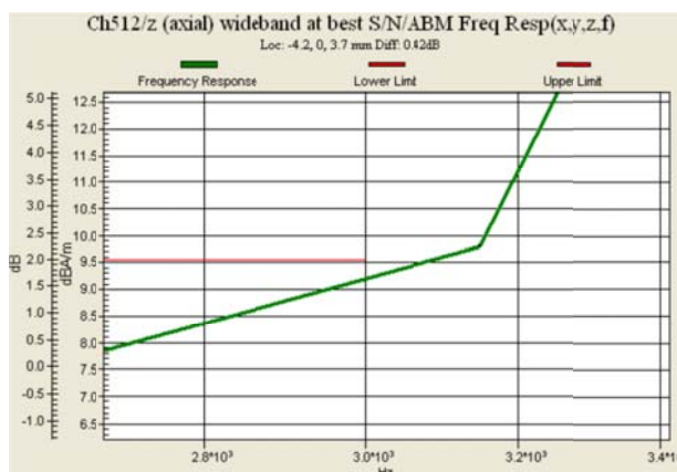
Fig 8.5 GSM1900 Ch512
