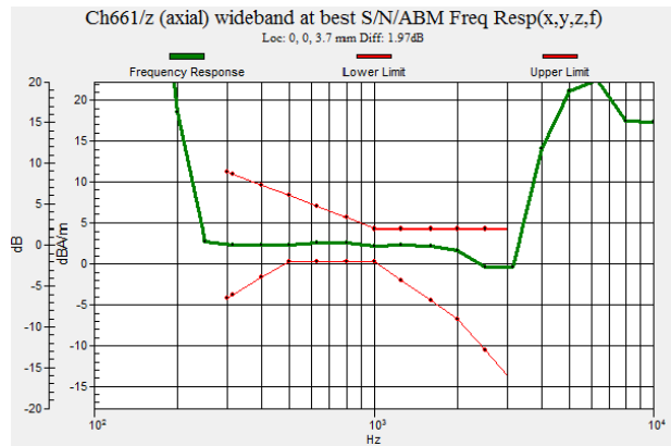
Fig 7.2 GSM1900 Ch661
