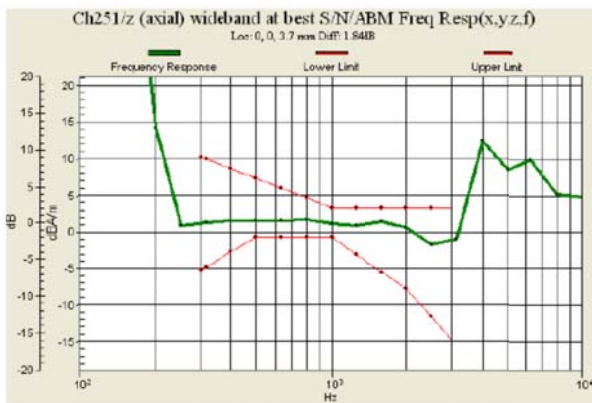
Fig 7.3 GSM850 Ch251
