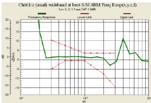
Fig 7.5 GSM1900 Ch661
