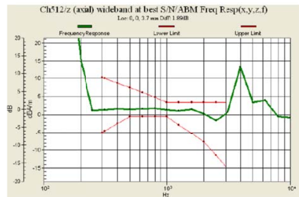
Fig 7.4 GSM1900 Ch512
