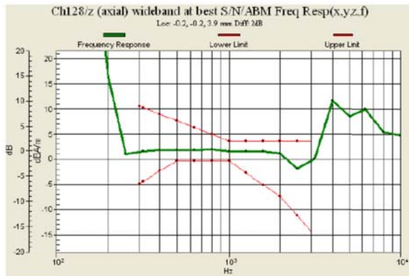
Fig 7.1 GSM850 Ch128
