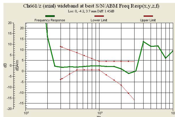
Fig 7.2 GSM1900 Ch661
