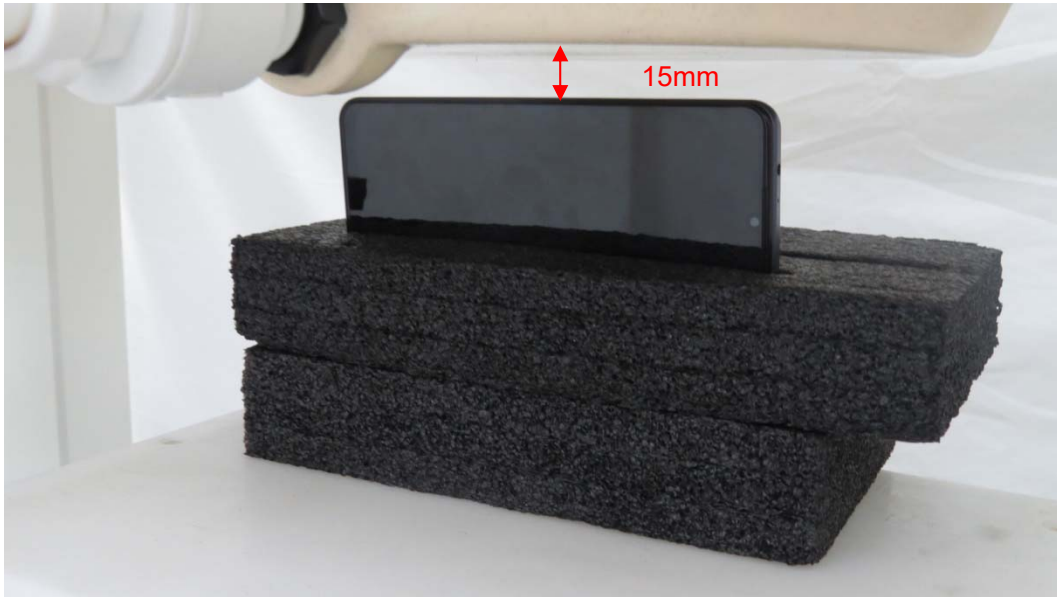
Picture 7: Left Edge, the distance from handset to the bottom of the Phantom is 15mm
