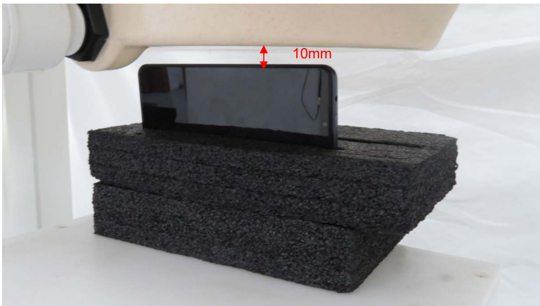
Picture 12: Left Edge, the distance from handset to the bottom of the Phantom is 10mm
