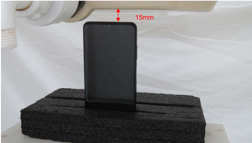
Picture 9: Top Edge, the distance from handset to the bottom of the Phantom is 15mm
