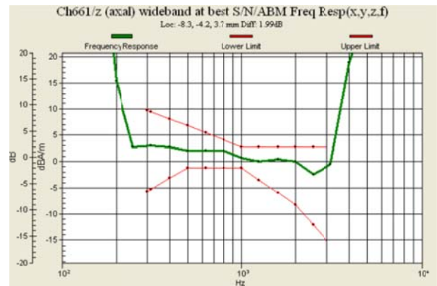
Fig 7.2 GSM1900 Ch661
