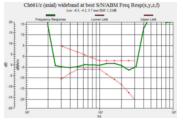
Fig 7.2 GSM1900 Ch661
