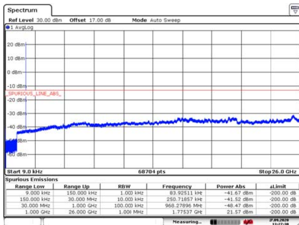
EN-DC_2A_n66 5MHz CH- High 9kHz~26GHz
