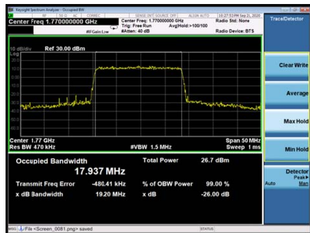
EN-DC_2A_n66 256QAM 20MHz CH-High
