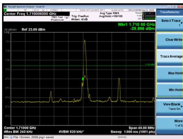
EN-DC_2A_n66 20MHz 256QAM 100%RB CH-Low
