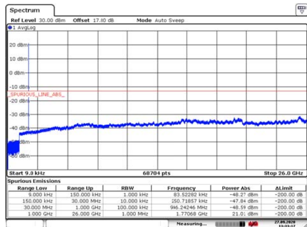
EN-DC_2A_n66 10MHz CH-High 9kHz~26GHz
