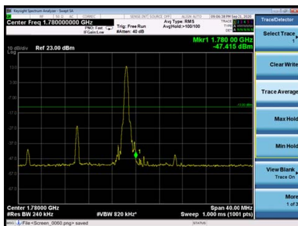
EN-DC_2A_n66 20MHz 256QAM 100%RB CH-High
