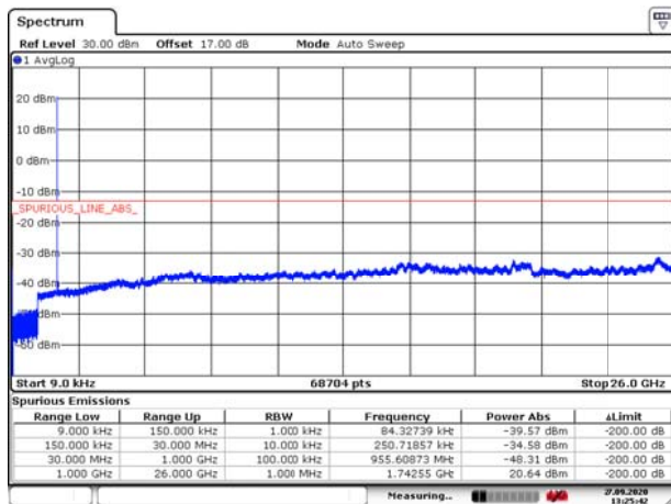
EN-DC_2A_n66 5MHz CH- Middle 9kHz~26GHz
