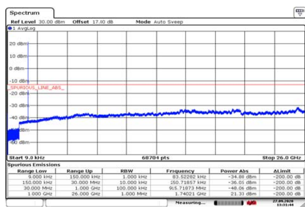
EN-DC_2A_n66 10MHz CH- Middle 9kHz~26GHz
