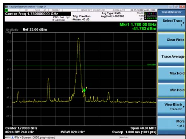
EN-DC_2A_n66 20MHz 16QAM 1RB CH-High
