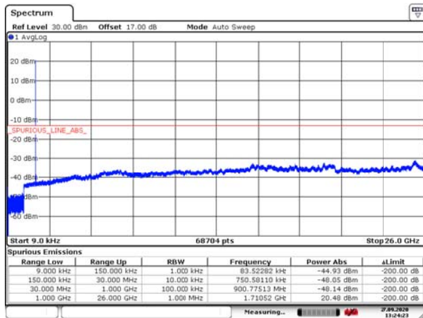
EN-DC_2A_n66 5MHz CH-Low 9kHz~26GHz
