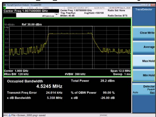
EN-DC_66A_n2 5MHz 256QAM CH-High
