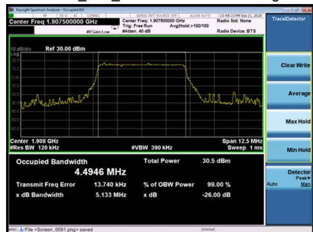
EN-DC_66A_n2 5MHz 16QAM CH-High
