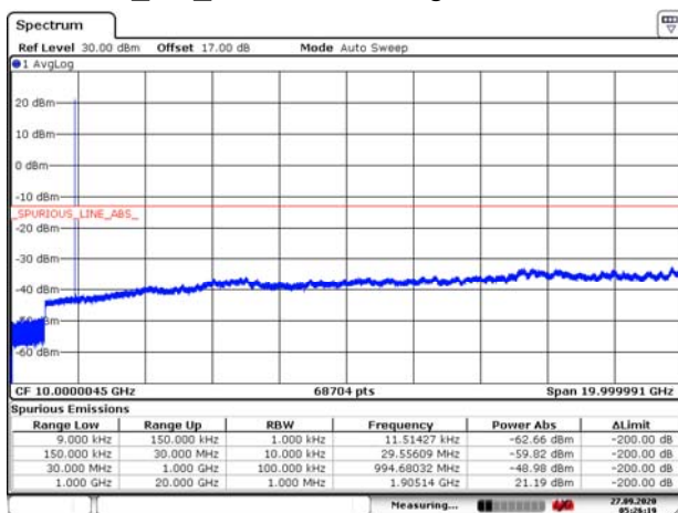
EN-DC_5A_n2 5MHz CH-High 9kHz~20GHz
