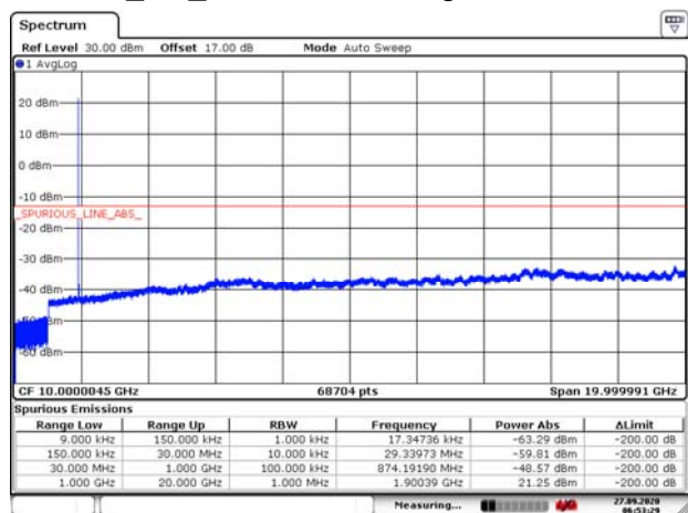
EN-DC_5A_n2 10MHz CH-High 9kHz~20GHz
