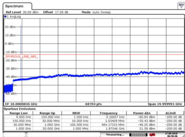
EN-DC_5A_n2 10MHz CH-Middle 9kHz~20GHz
