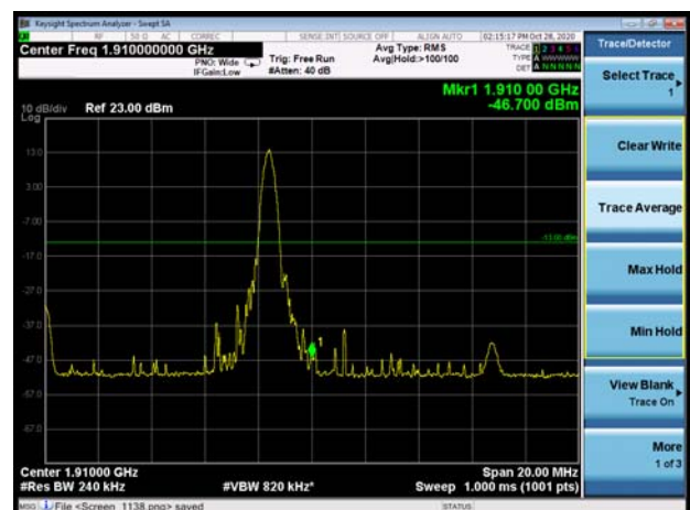
EN-DC_66A_n2 20MHz 16QAM 1RB CH-High
