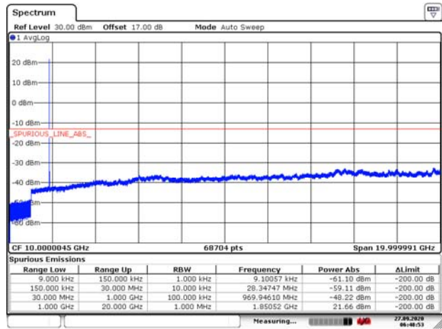
EN-DC_5A_n2 10MHz CH-Low 9kHz~20GHz
