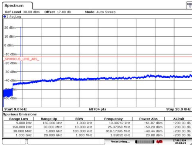
EN-DC_5A_n2 5MHz CH-Low 9kHz~20GHz
