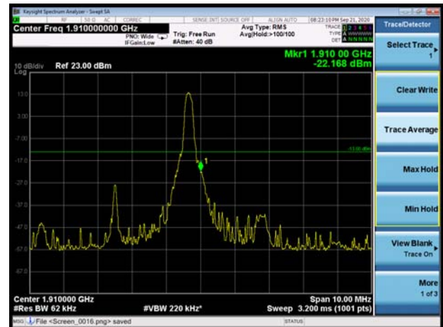
EN-DC_66A_n2 5MHz 64QAM 100%RB CH-High
