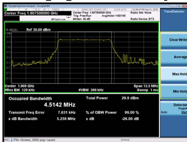
EN-DC_66A_n2 5MHz 64QAM CH-High
