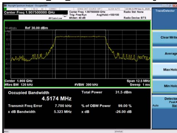
EN-DC_66A_n2 5MHz QPSK CH-High
