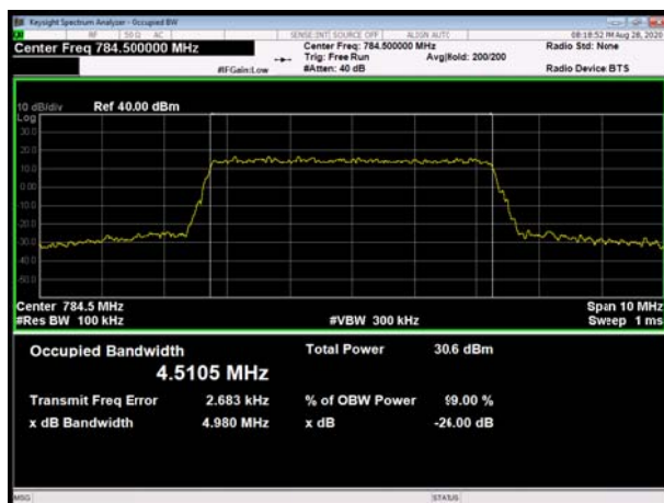
LTE Band 13 64QAM 5MHz CH-High
