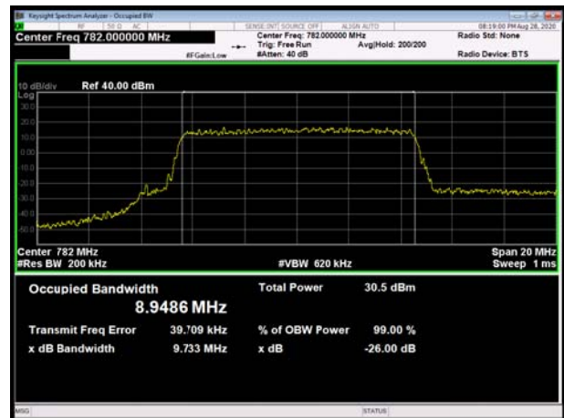
LTE Band 13 16QAM 10MHz CH-Middle
