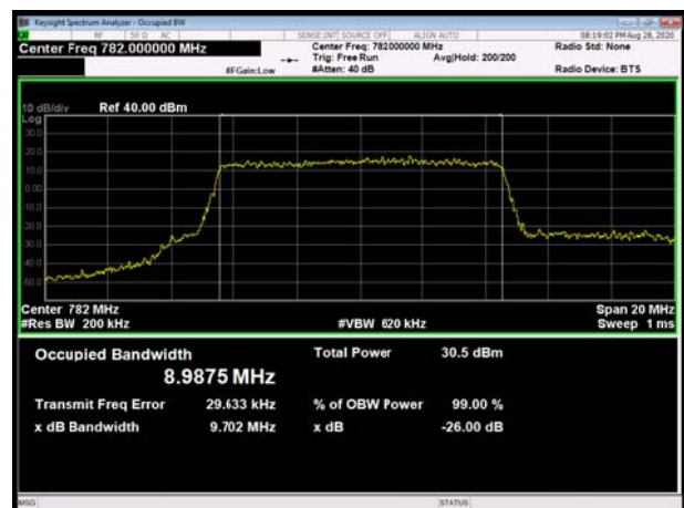
LTE Band 13 64QAM 10MHz CH-Middle
