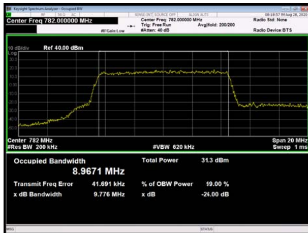
LTE Band 13 QPSK 10MHz CH-Middle
