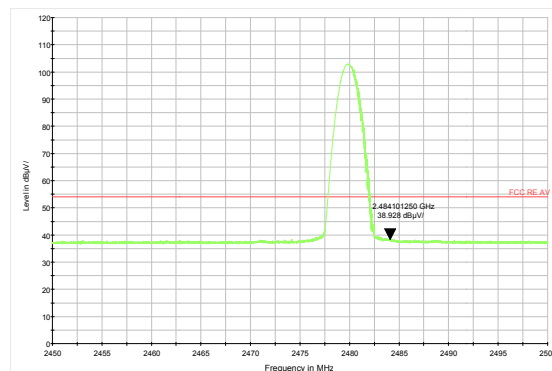
DH5-Channel 78: Average
