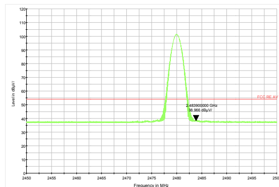
3DH5-Channel 78: Average
