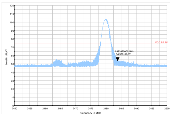
DH5-Channel 78: Peak
