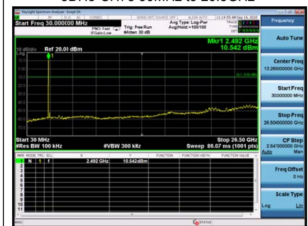
3DH5-CH78 30MHz to 26.5GHz
