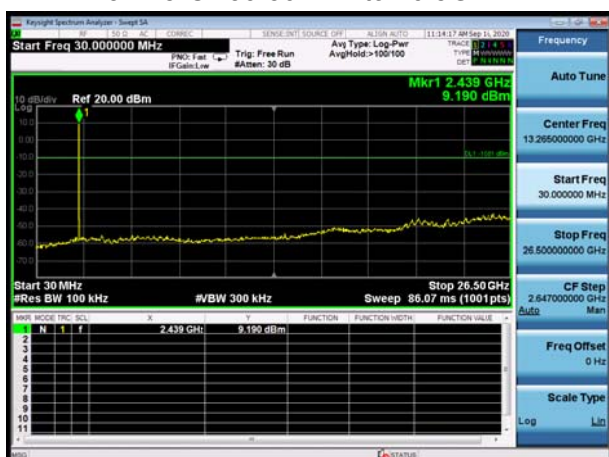
3DH5-CH39 30MHz to 26.5GHz
