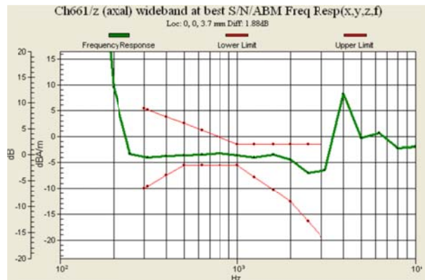
Fig 7.2 GSM1900 Ch661
