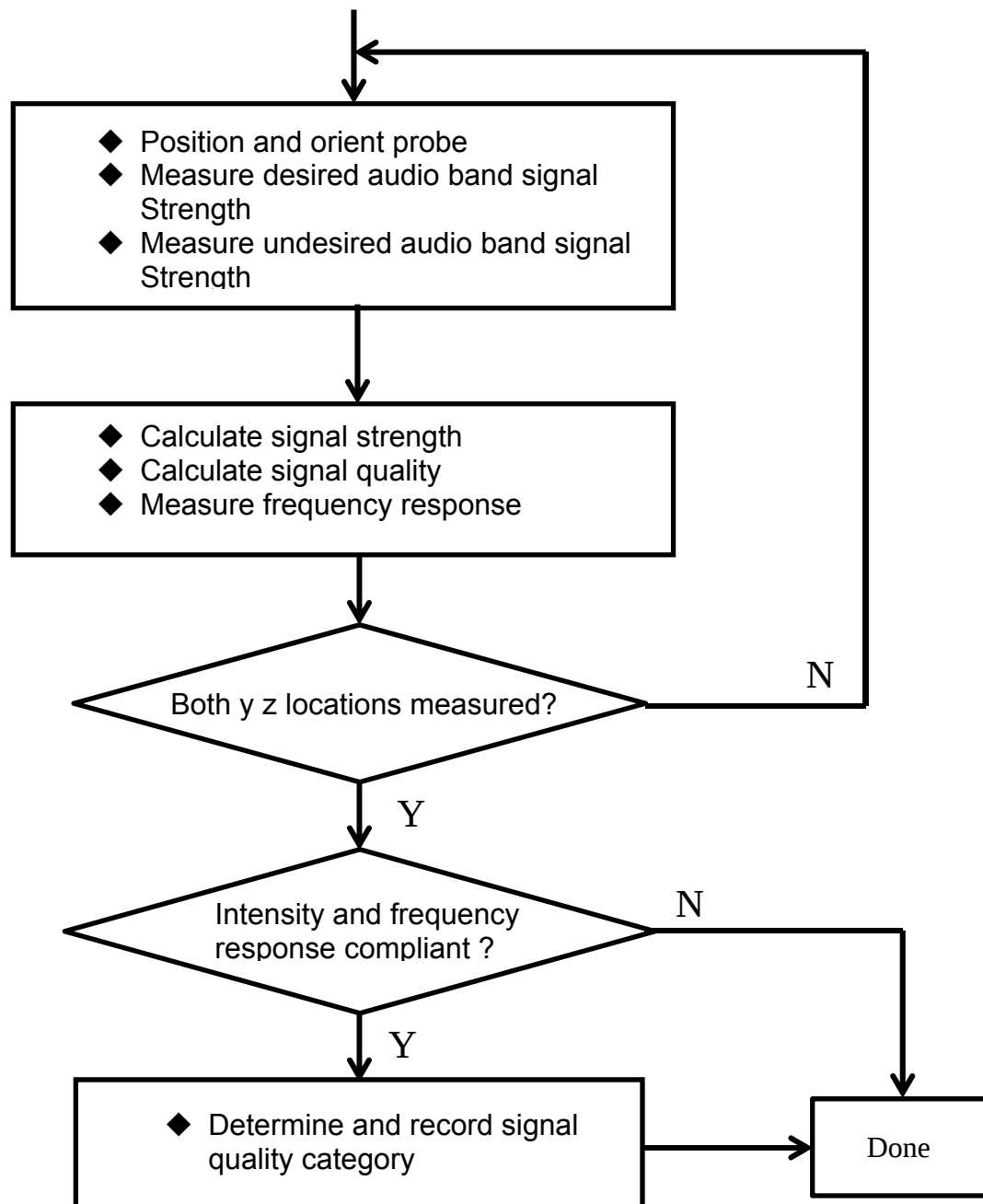
Fig. 6.1 Test Flow Chart
