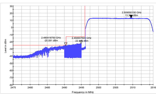
LTE Band 41 QPSK 20MHz CH-Low, 100%RB
