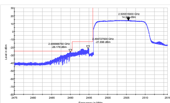
LTE Band 41 QPSK 15MHz CH-Low, 100%RB
