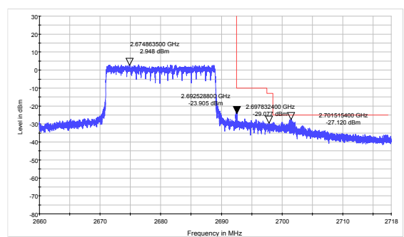
LTE Band 41 16QAM 20MHz CH-High, 100%RB
