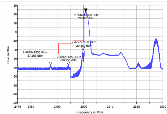
LTE Band 7 16QAM 15MHz CH-Low, 100%RB
