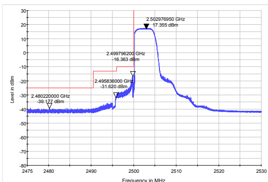
LTE Band 7 QPSK 10MHz CH-Low, 1 RB
