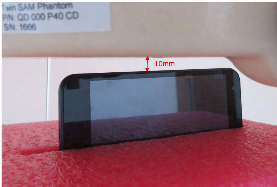
Picture 21: Right Side, the distance from handset to the bottom of the Phantom is 10mm
