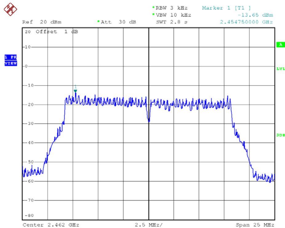
802.11g - Channel 11
