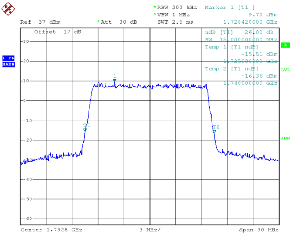
99% Occupied Bandwidth LTE Band 4/15MHz/16QAM
