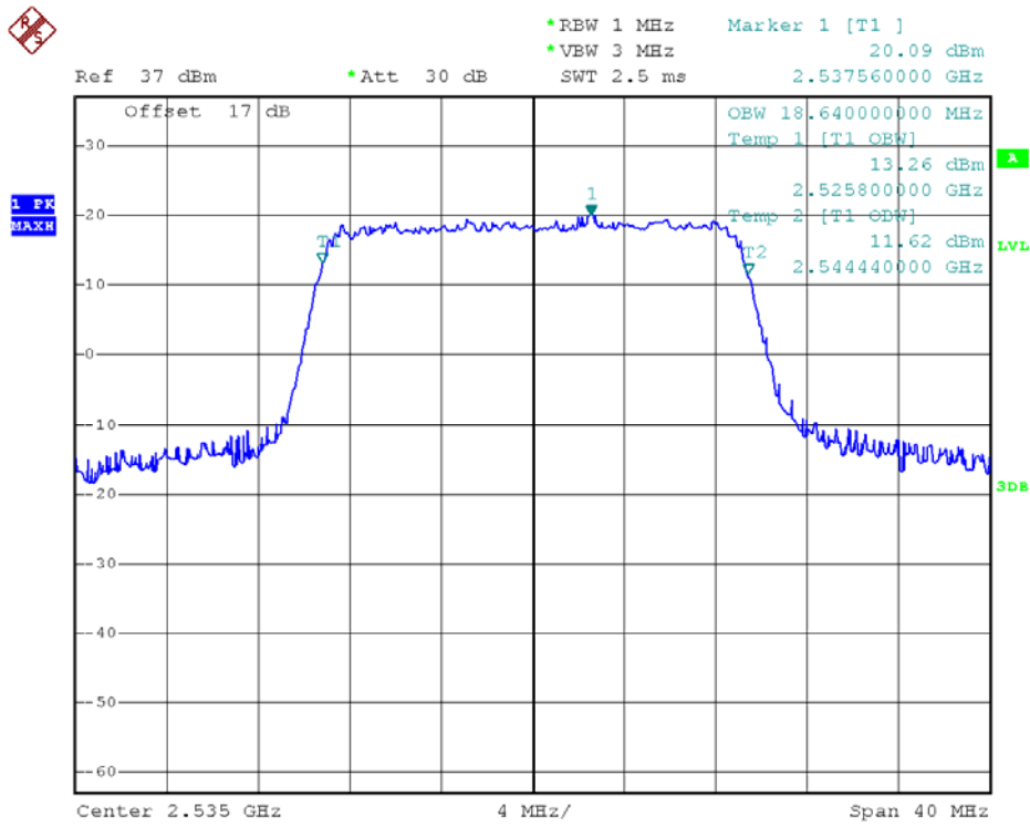
99% Occupied Bandwidth LTE Band 7/20MHz/QPSK
