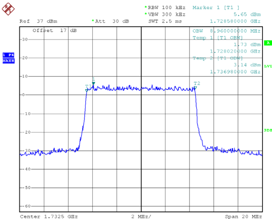
99% Occupied Bandwidth LTE Band 4/10MHz/16QAM
