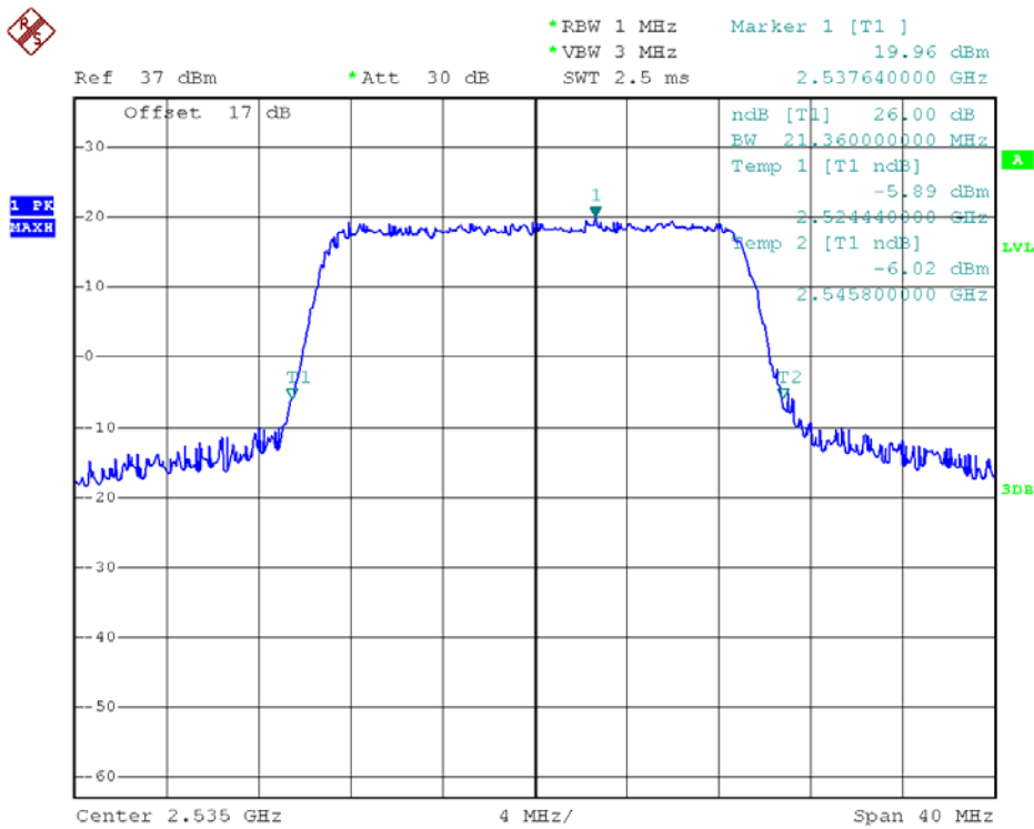
26dB Bandwidth LTE Band 7/20MHz/QPSK
