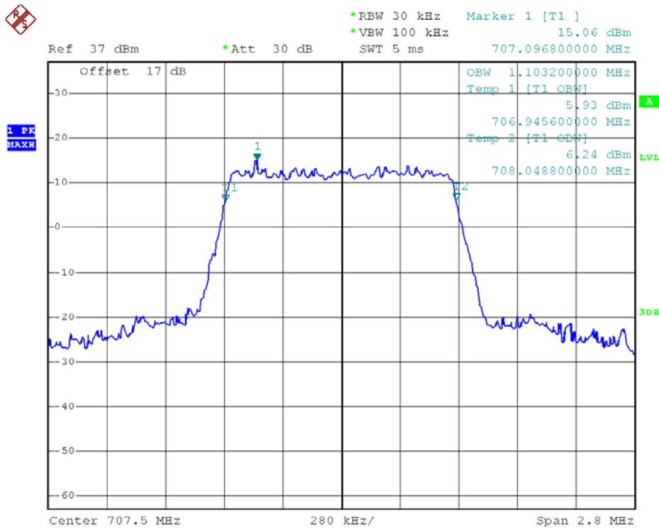
99% Occupied Bandwidth LTE Band 12/1.4MHz/16QAM
