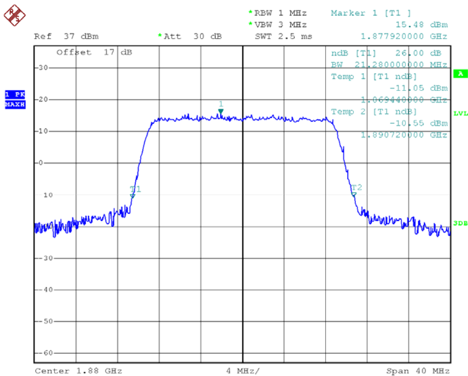
99% Occupied Bandwidth LTE Band 2/20MHz/16QAM
