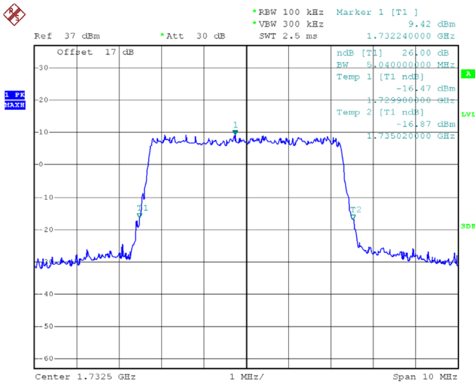
26dB Bandwidth LTE Band 4/5MHz/QPSK
