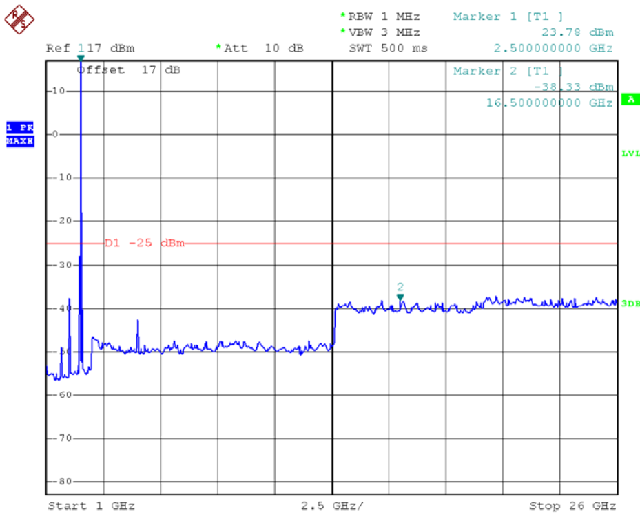
RB Size 1, RB Offset 0 1GHz to 26GHz
