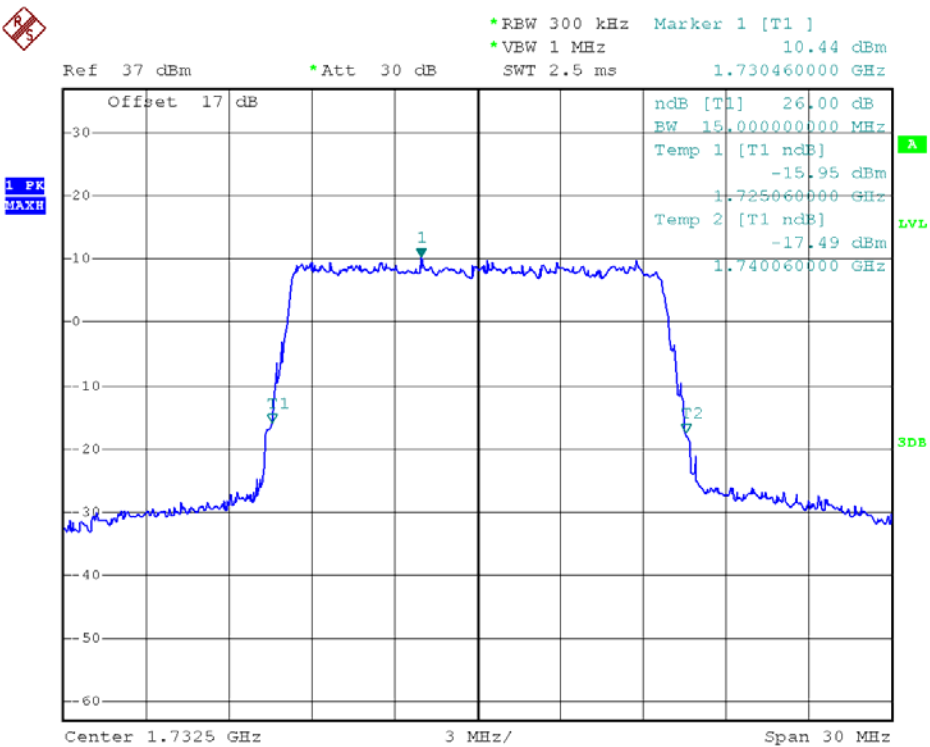
26dB Bandwidth LTE Band 4/15MHz/QPSK
