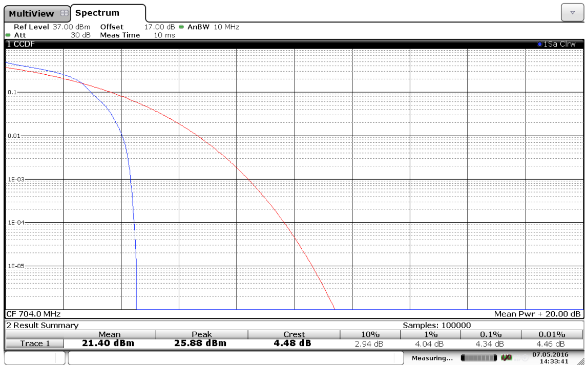
(Plot D1: Band 12/10MHz/16QAM in L Ch 1RB Size )
