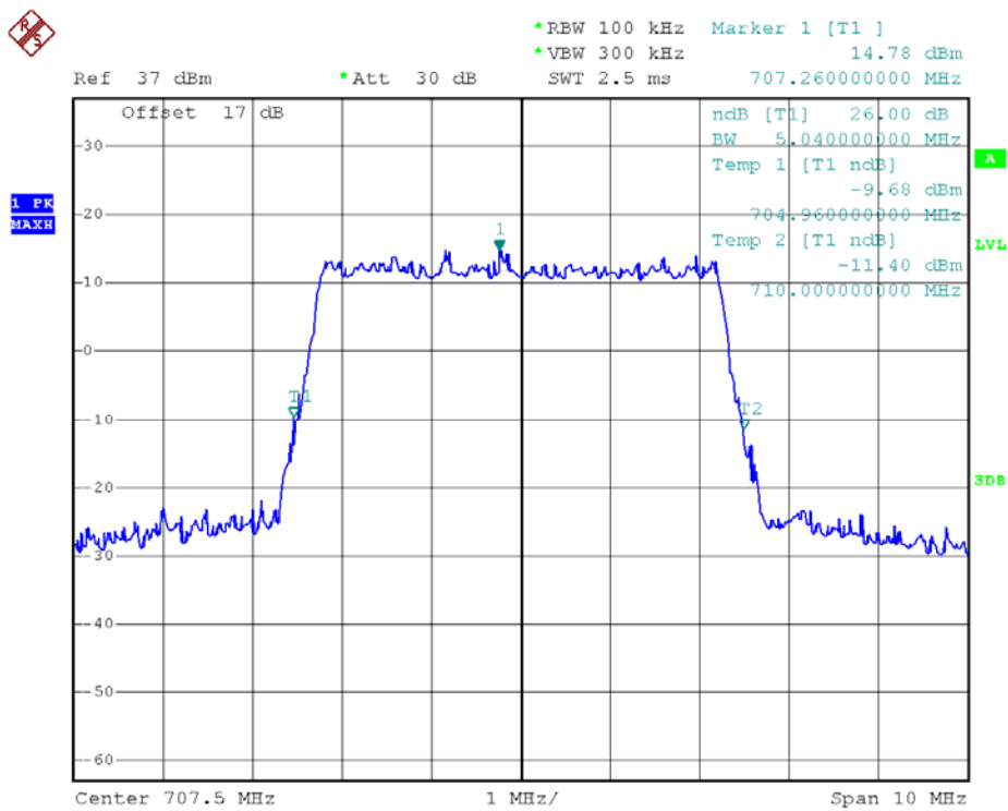
99% Occupied Bandwidth LTE Band 12/5MHz/QPSK
