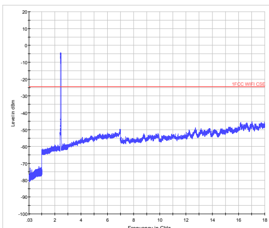
802.11n (HT40) CH11 30MHz to 18GHz
