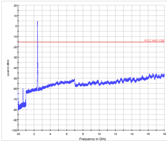
802.11n (HT40) CH1 30MHz to 18GHz
