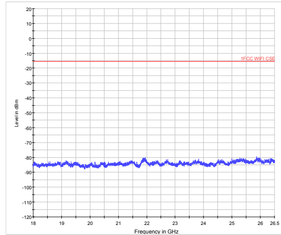
802.11n (HT40) CH1 18GHz to 26.5GHz
