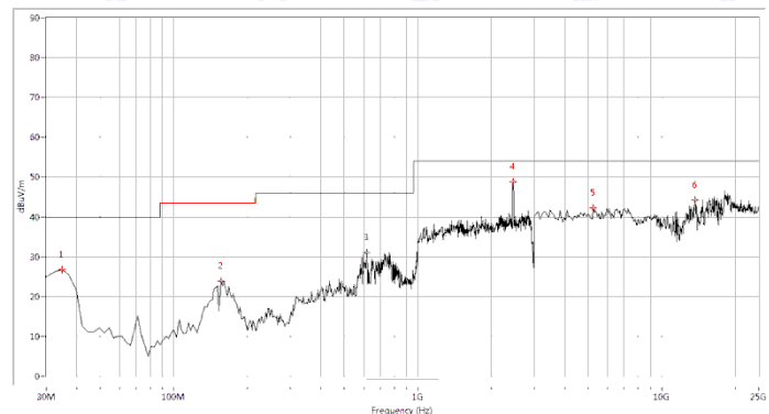
(Plot C.2: Antenna Horizontal, 30MHz to 25GHz)
