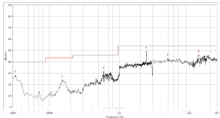
(Plot B.2: Antenna Horizontal, 30MHz to 25GHz)
