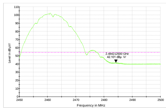
802.11b-Channel 11 Average
