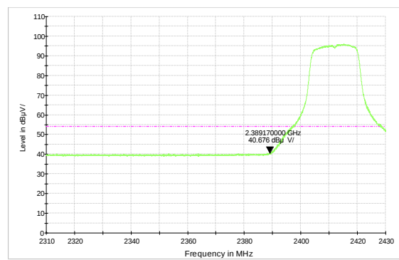
802.11g-Channel 1 Average
