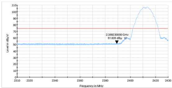
802.11b-Channel 1 Peak
