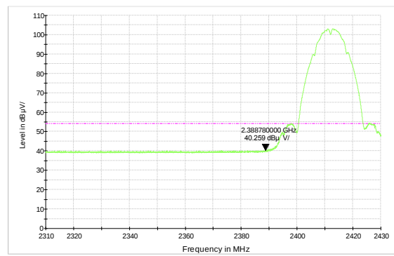
802.11b-Channel 1 Average
